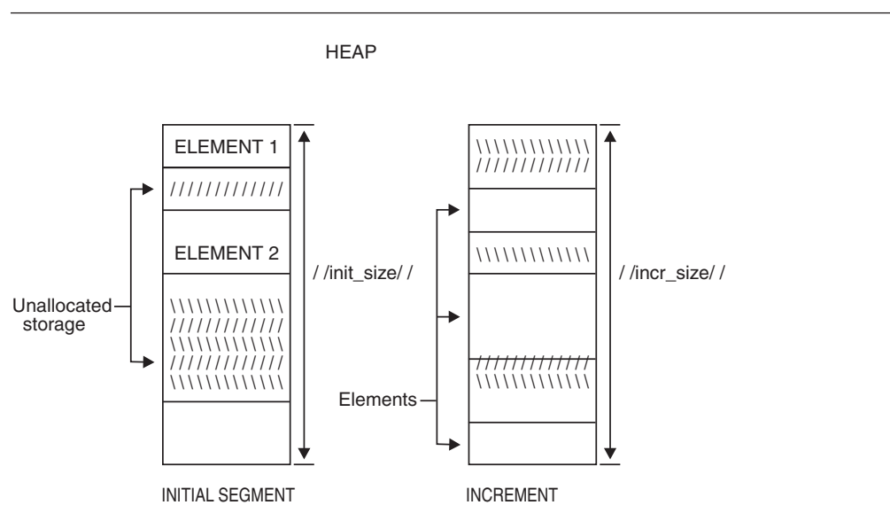
Figure 57. Language Environment Heap Storage Model
