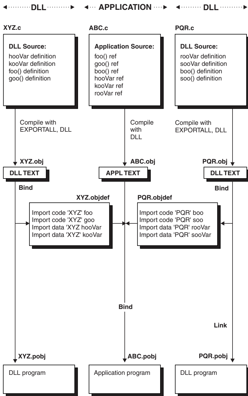
Figure 28. Summary of DLL and DLL Application Preparation and Usage
