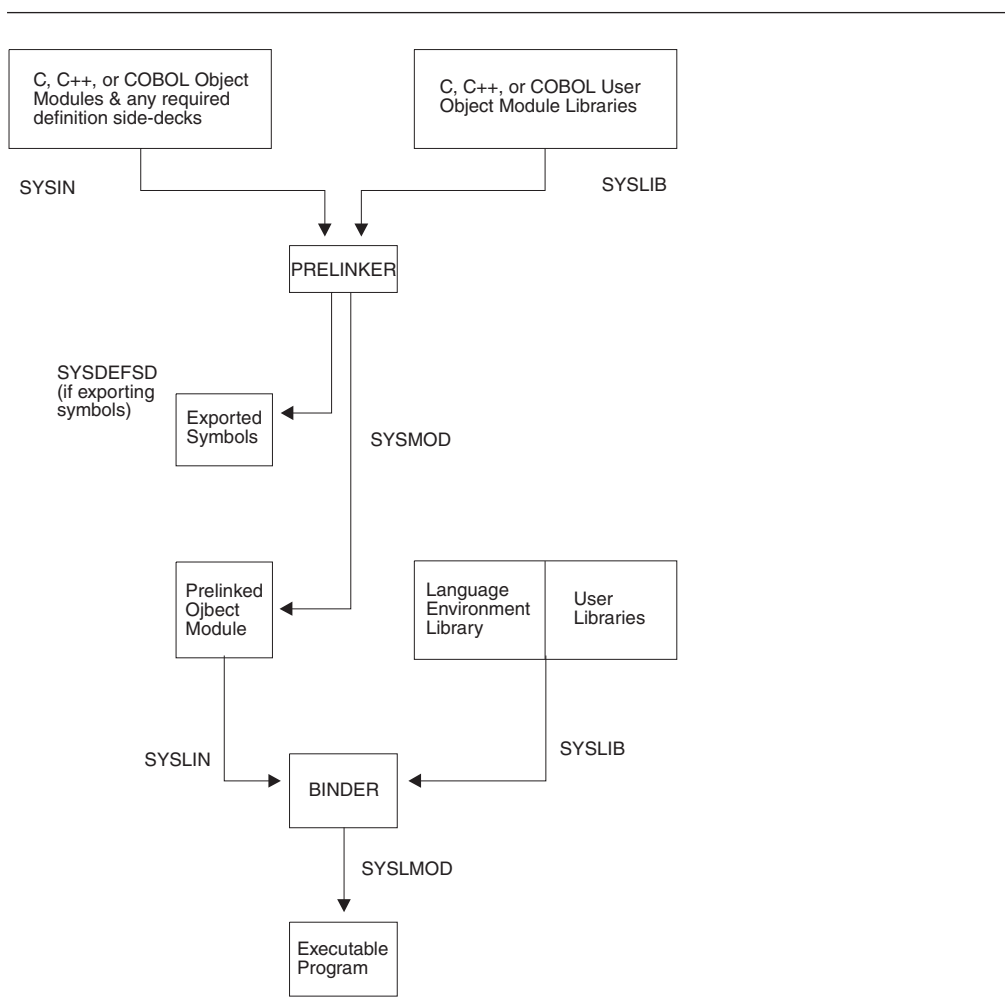
Figure 176. Basic Prelinker and Linkage Editor Processing
